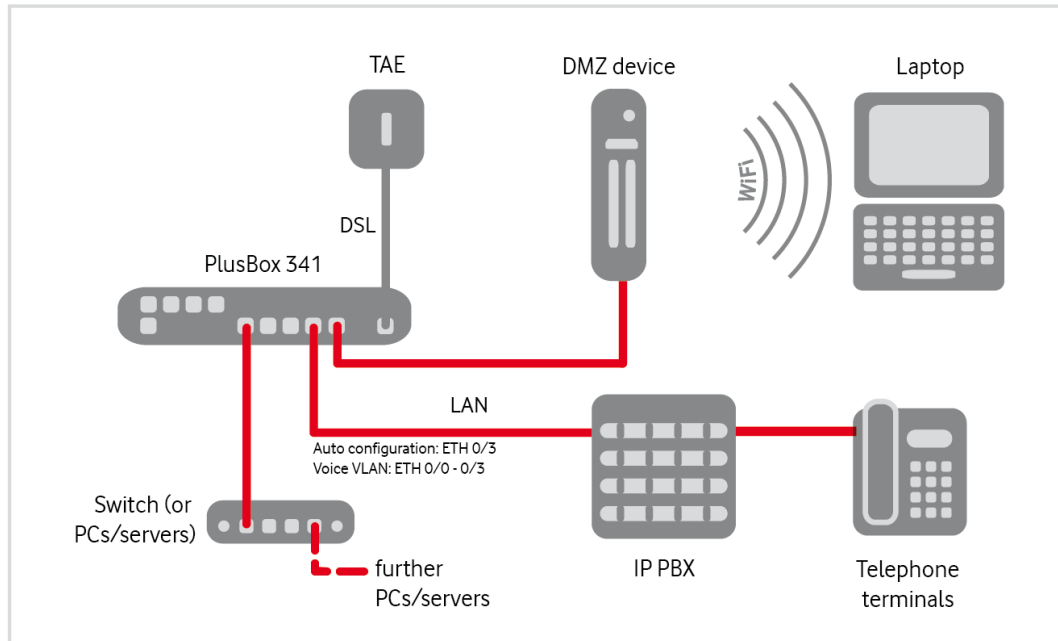
Fig. 7: Anlagen-Anschluss Plus, Connecting hardware with PlusBox 341, IP Voice + Data – Overview
