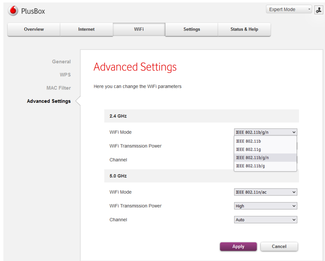
Fig. 38: PlusBox 341, Advanced Settings content page
