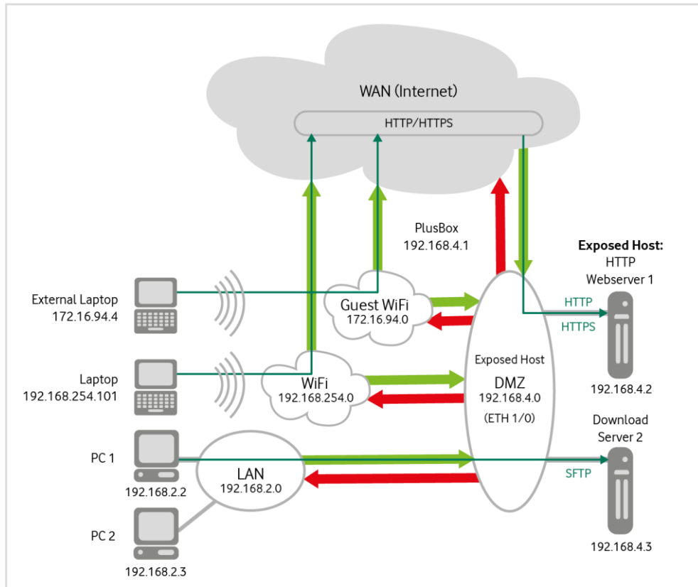
Fig. 73: PlusBox 341, Sample configuration web server in DMZ
