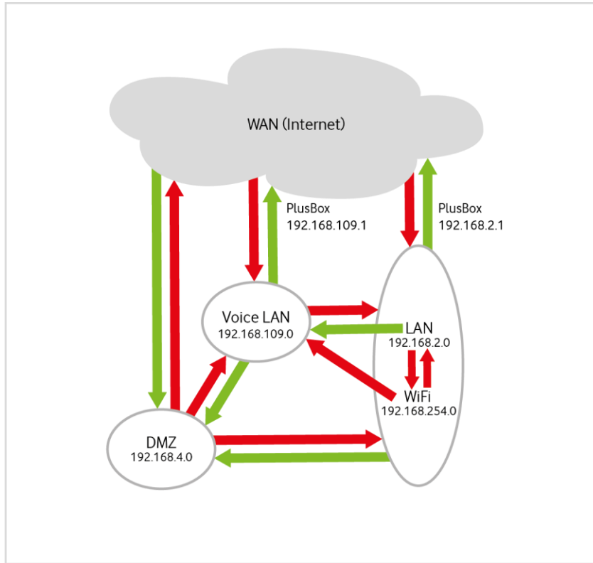
Fig. 60: PlusBox 341, Default firewall configuration for Voice LAN (IP Voice + Data)
