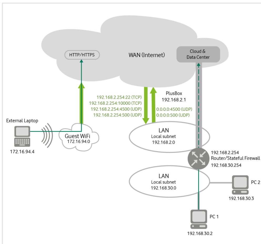
Fig. 74: PlusBox 341, Sample configuration VPN router in the LAN
