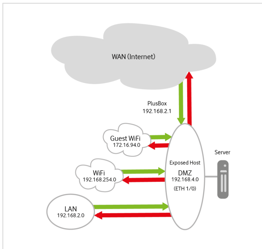
Fig. 65: PlusBox 341, DMZ/Exposed Host default configuration
