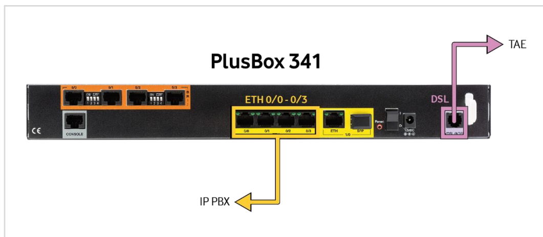
Fig. 6: Anlagen-Anschluss Plus, Connecting hardware with PlusBox 341, IP Voice only – Detail
