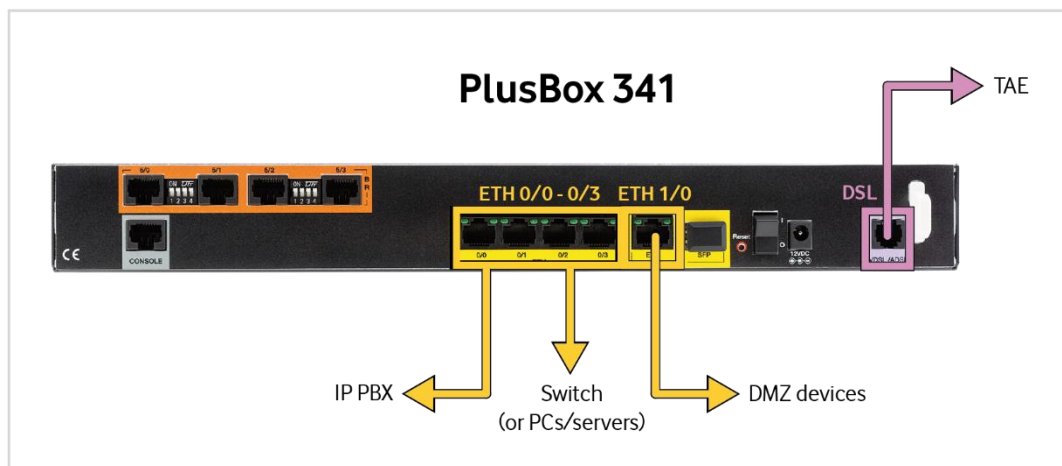
Fig. 9: Anlagen-Anschluss Plus, Connecting hardware with PlusBox 341, IP Voice + Data – VLAN config. detail
