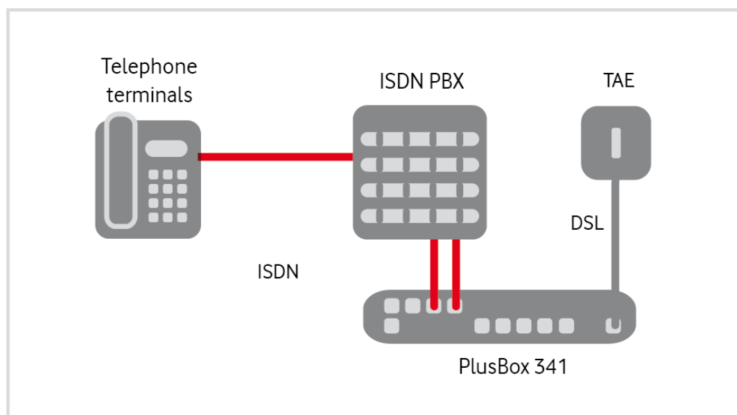
Fig. 3: Anlagen-Anschluss Plus, Connecting hardware with PlusBox 341, ISDN Voice only – Overview
