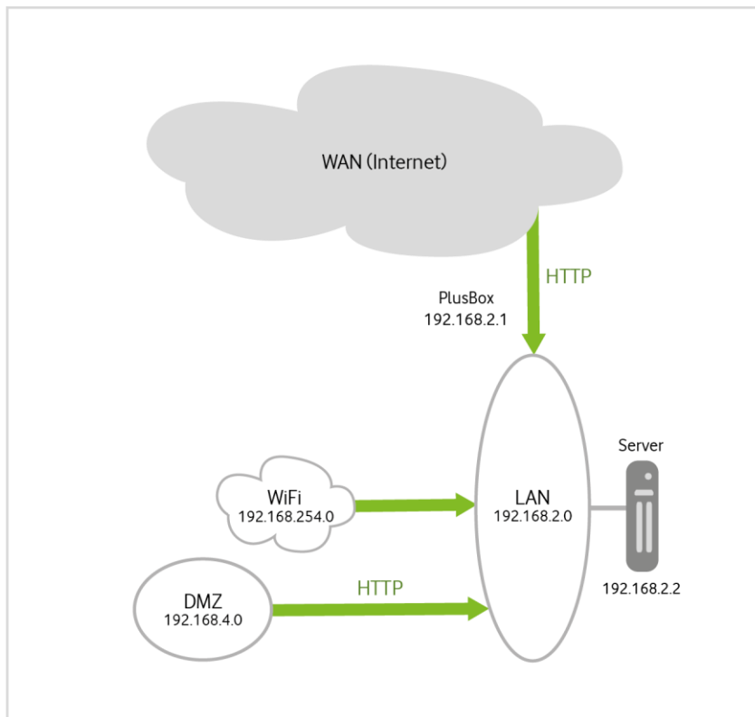
Fig. 61: PlusBox 341, HTTP server in the LAN – sample configuration
