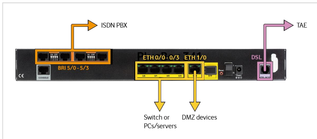
Fig. 2 : Anlagen-Anschluss Plus, Connecting hardware with PlusBox 341, ISDN Voice + Data – Detail
