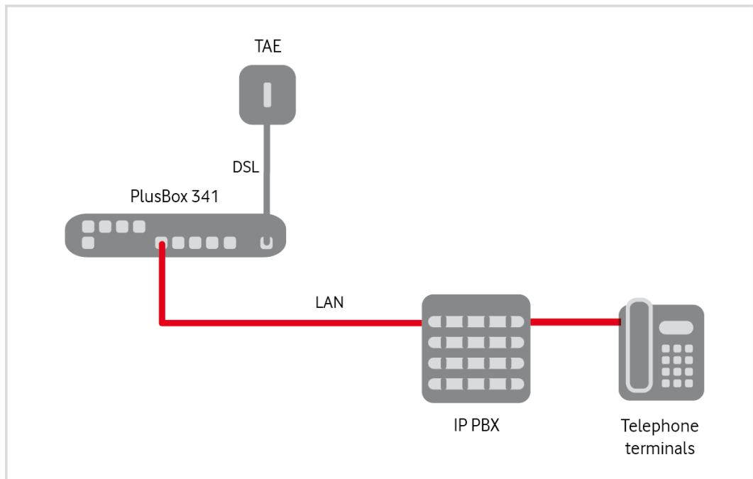
Fig. 5: Anlagen-Anschluss Plus, Connecting hardware with PlusBox 341, IP Voice only – Overview
