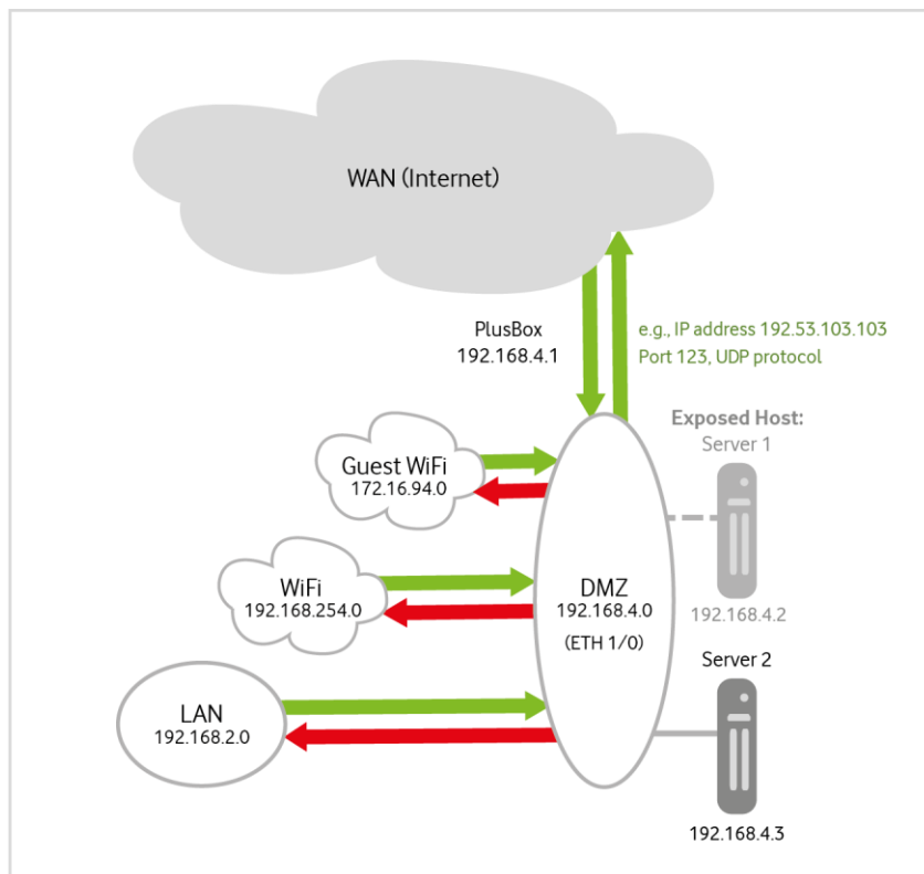
Fig. 71: PlusBox 341, DMZ computer uses Internet NTP server – sample configuration
