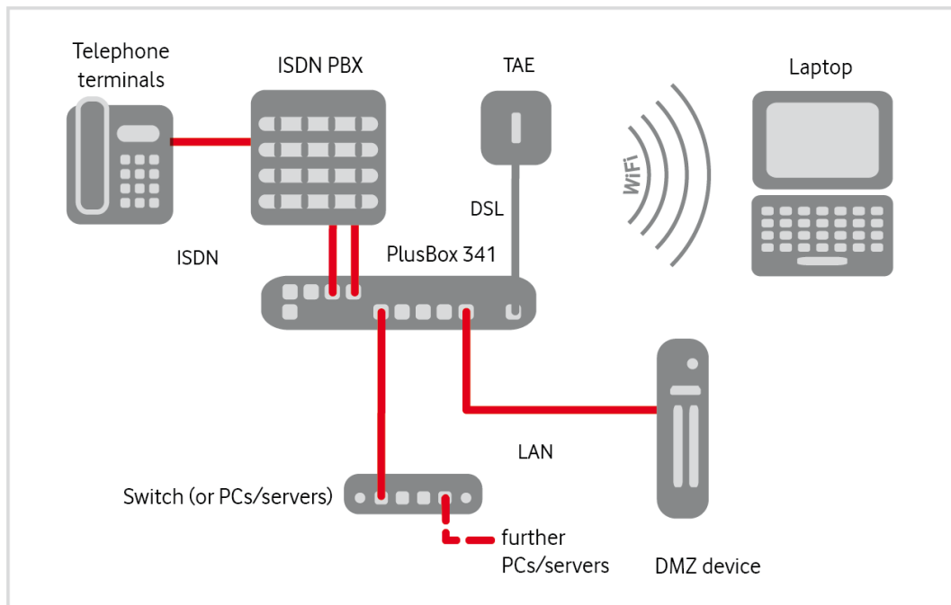
Fig. 1: Anlagen-Anschluss Plus, Connecting hardware with PlusBox 341, ISDN Voice + Data – Overview
