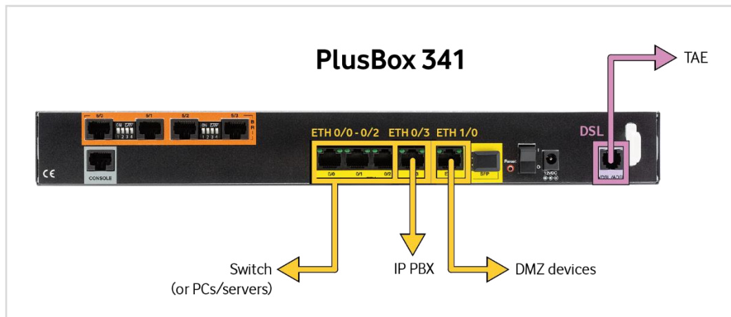
Fig. 8: Anlagen-Anschluss Plus, Connecting hardware with PlusBox 341, IP Voice + Data – Auto configuration detail
