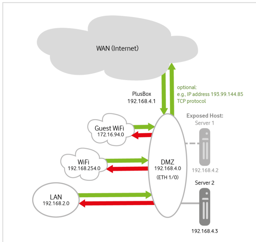
Fig. 66: PlusBox 341, Software download via DMZ host – sample configuration
