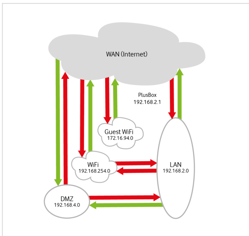
Fig. 59: PlusBox 341, Default firewall configuration for LAN (ISDN/IP Voice + Data)
