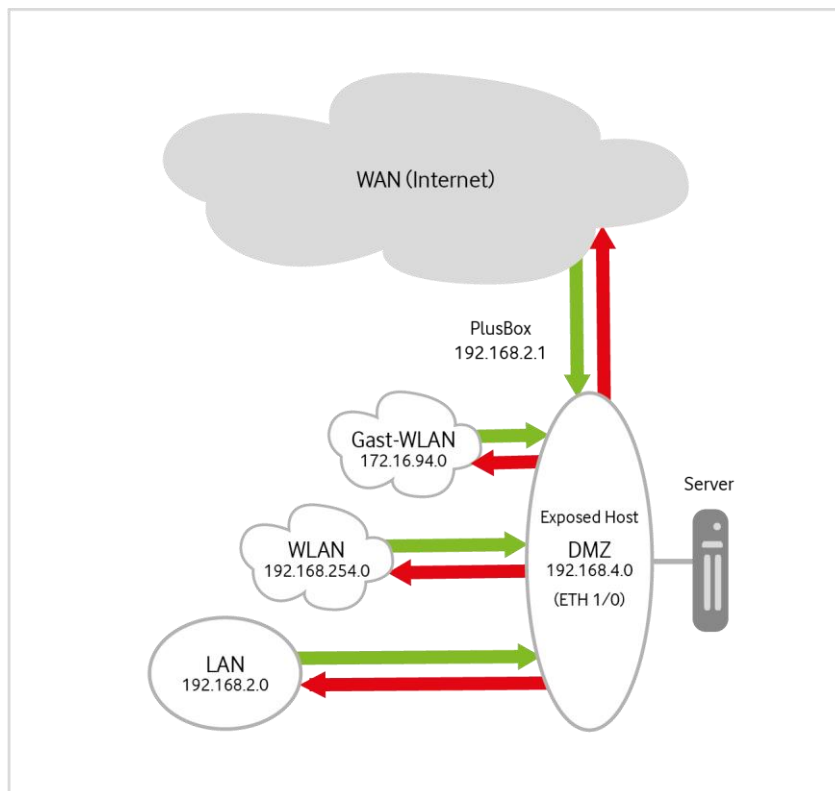
Abb. 65: PlusBox 341, Standardkonfiguration DMZ/Exposed Host
